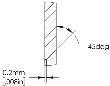
DETAIL B
