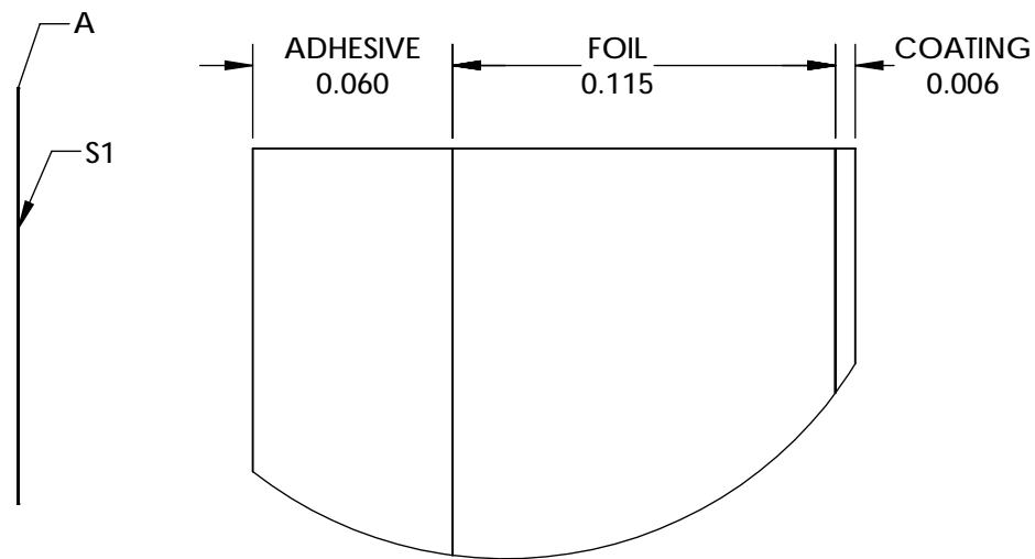
DETAIL A
