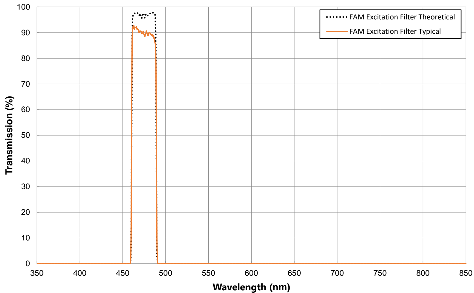
475nm CWL, OD8 High Blocking Bandpass Filter FOR REFERENCE ONLY
