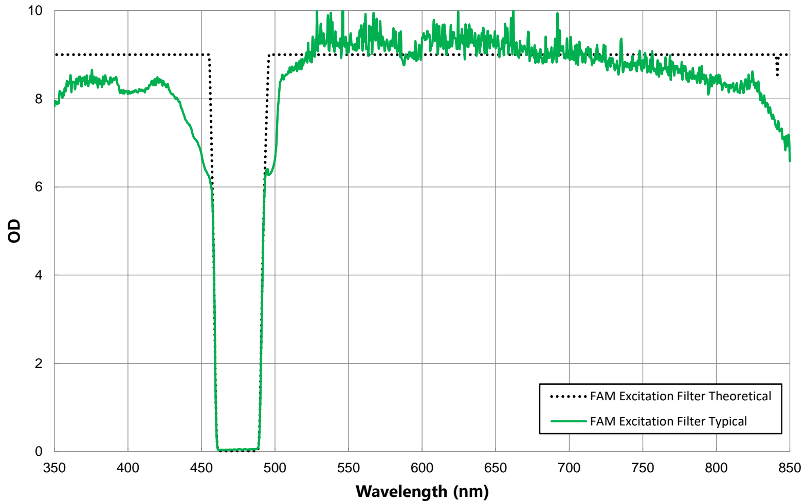
475nm CWL, OD8 High Blocking Bandpass Filter FOR REFERENCE ONLY
