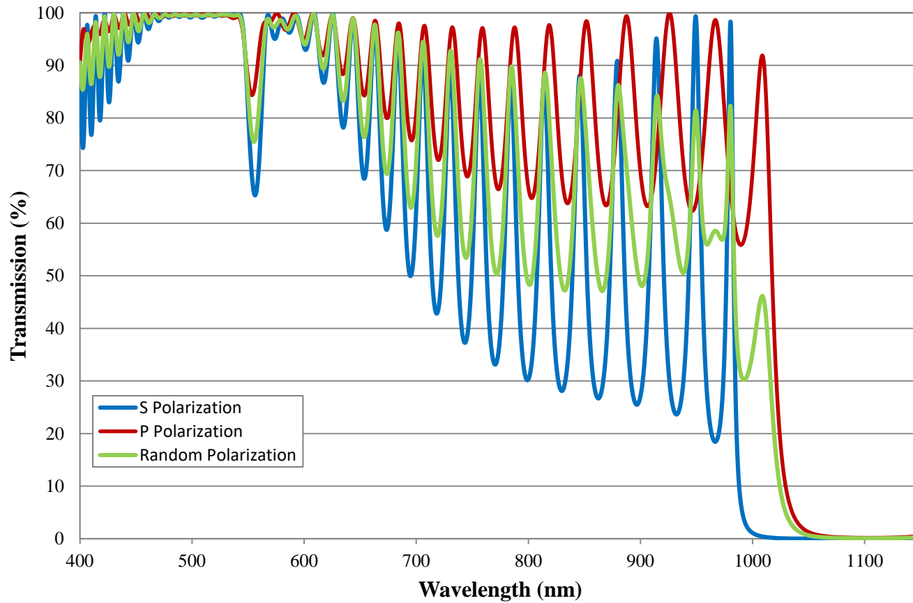
532nm T, 1064nm R Harmonic Separator Typical Transmission FOR REFERENCE ONLY
