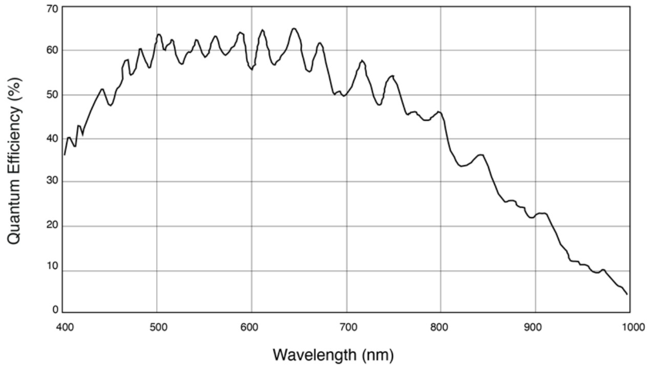
MT9P031 Sensor QE Curve
