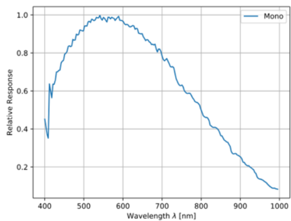
E2525A Sensor QE Curve
