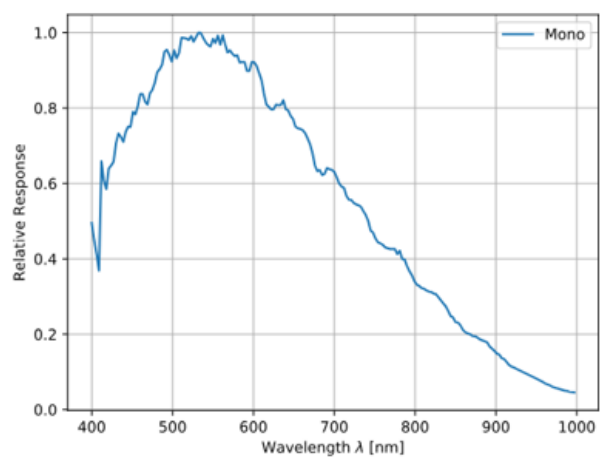
GMAX2505 Sensor QE Curve
