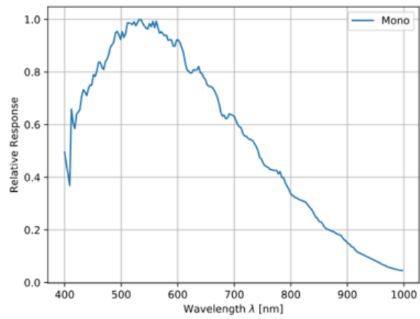
GMAX2518 Sensor QE Curve
