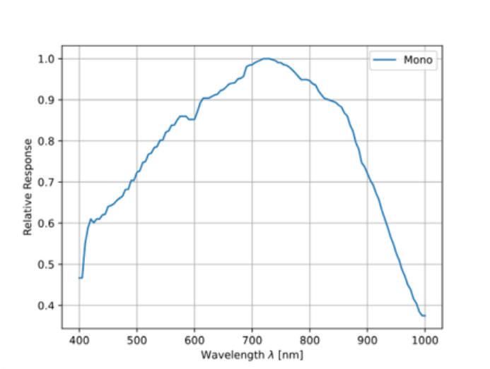
IMX676 Sensor QE Curve
