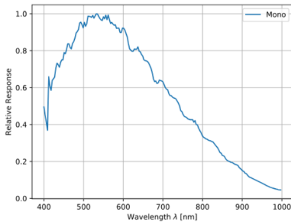
GMAX2509 Sensor QE Curve
