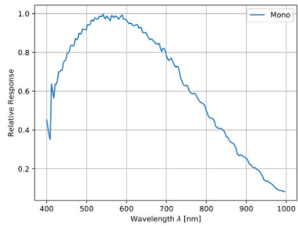
IMX547 Sensor QE Curve
