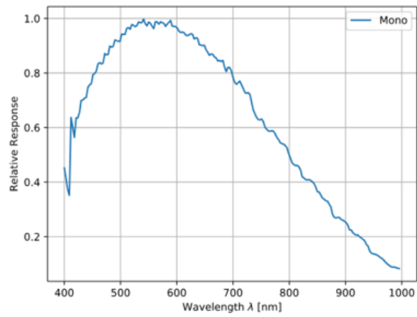
IMX545 Sensor QE Curve
