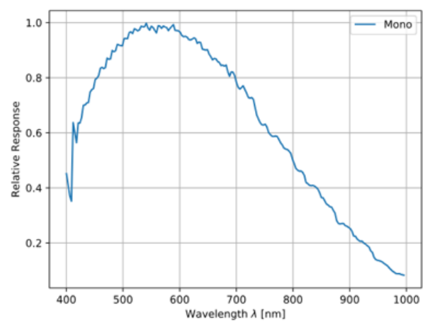
IMX546 Sensor QE Curve
